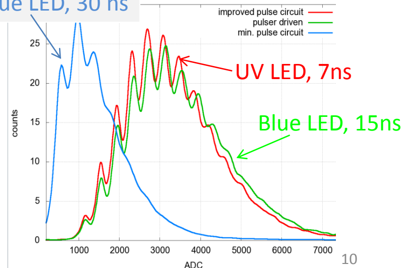
Blue LED, 30 ns
