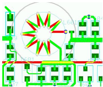
Special PCB toroidal inductors for low RFI ( \sim 35\text{nH} )
